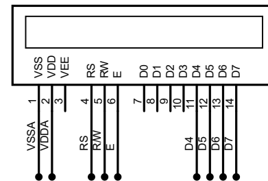
LCD1 LM020L
